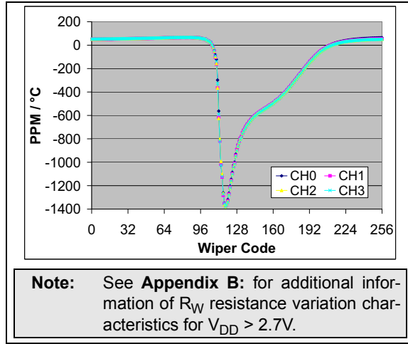
FIGURE 2-41: 10 kΩ – R_{WB} PPM/°C vs. Wiper Setting. ( R_{BW(\text{code}=n, 125^\circ\text{C})} - R_{BW(\text{code}=n, -40^\circ\text{C})} / R_{BW(\text{code}=256, 25^\circ\text{C}) / 165^\circ\text{C} * 1,000,000 ) ( V_{DD} = 1.8\text{V} , I_W = 150\text{ }\mu\text{A} ).
