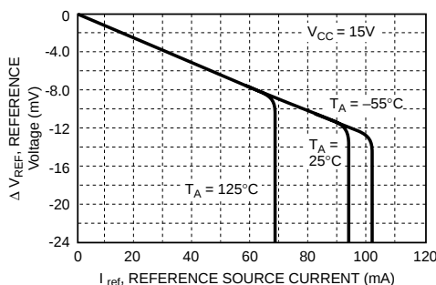
Reference Voltage Change vs. Source Current
