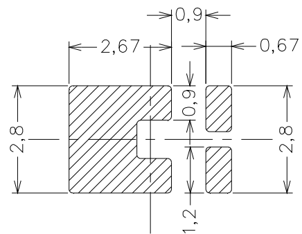
Soldering patterns
