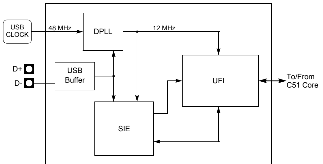
Figure 63. USB Connection
