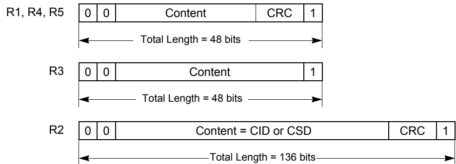
Figure 88. Response Token Format
