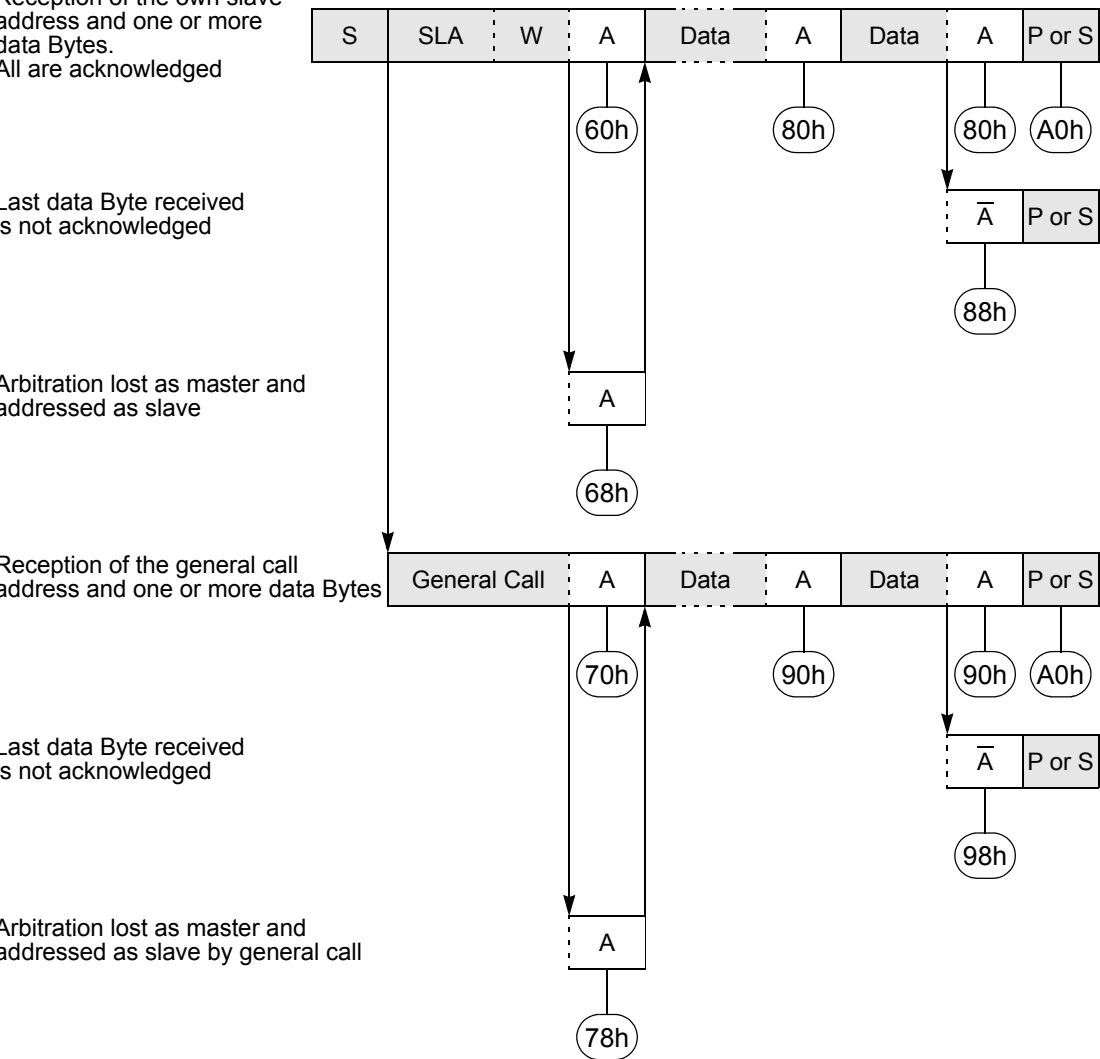
Figure 135. Format and States in the Slave Receiver Mode
