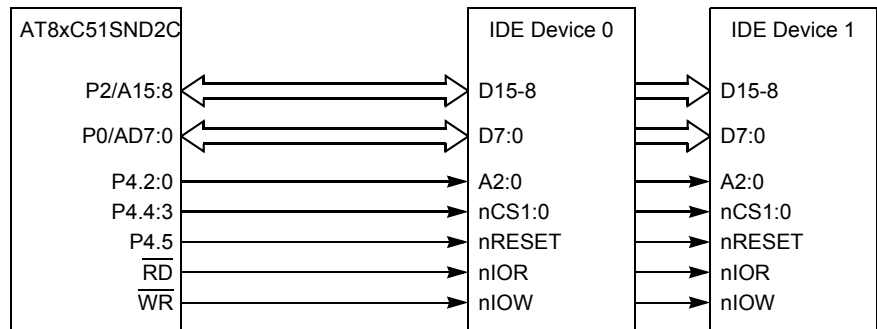
Figure 81. IDE Device Connection Example 2
