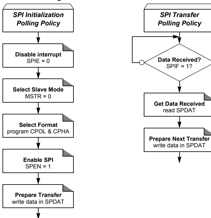
Figure 112. Slave SPI Polling Flows
