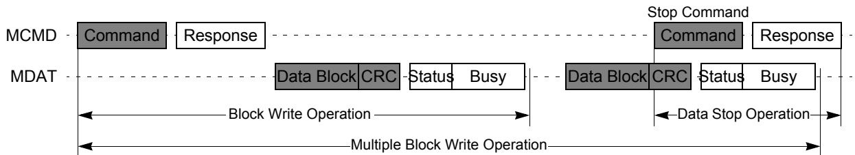
Figure 85. Multiple Block Write Operation
