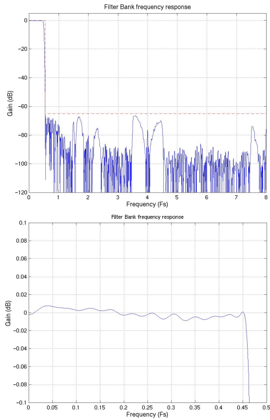
Figure 149. Channel Filter
