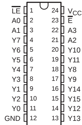
CD74HCT4514 . . . E PACKAGE CD74HCT4515 . . . E OR EN PACKAGE (TOP VIEW)
