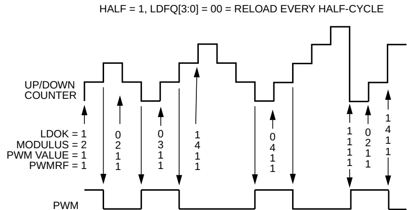
Figure 11-71. Half-Cycle Center-Aligned Modulus Loading
