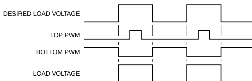
Figure 11-60. Correction with Negative Current
