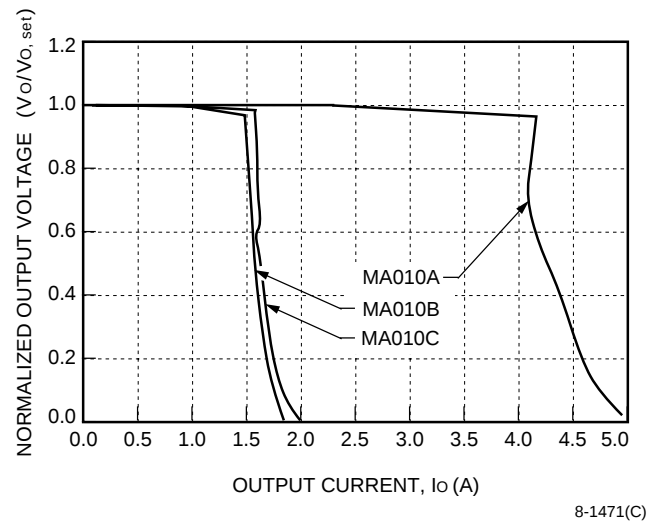
Figure 4. MA010A, B, C Typical Output Characteristics with V_i = 12\text{ V} , T_A = 25^\circ\text{C}
