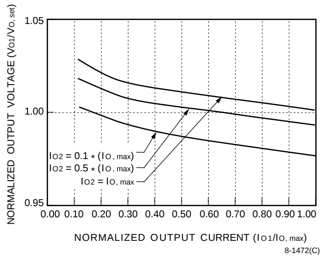
Figure 3. MA010BK, CL Typical Regulation: V_o vs. I_o for V_i = 12\text{ V} , T_c = 25^\circ\text{C}
