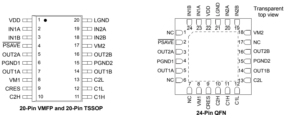
Figure 3. Pin Connections
