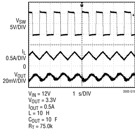
Operating Waveforms
