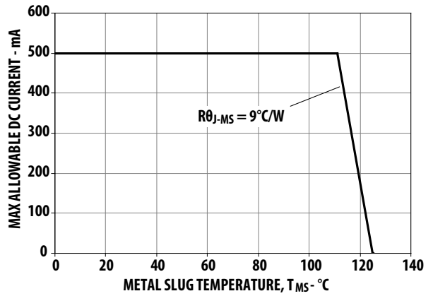
Figure 11. Maximum Forward Current vs. Ambient Slug Temperature. Derated based on T_{JMAX} = 125^\circ\text{C} , R_{\theta JMS} = 9^\circ\text{C/W}
