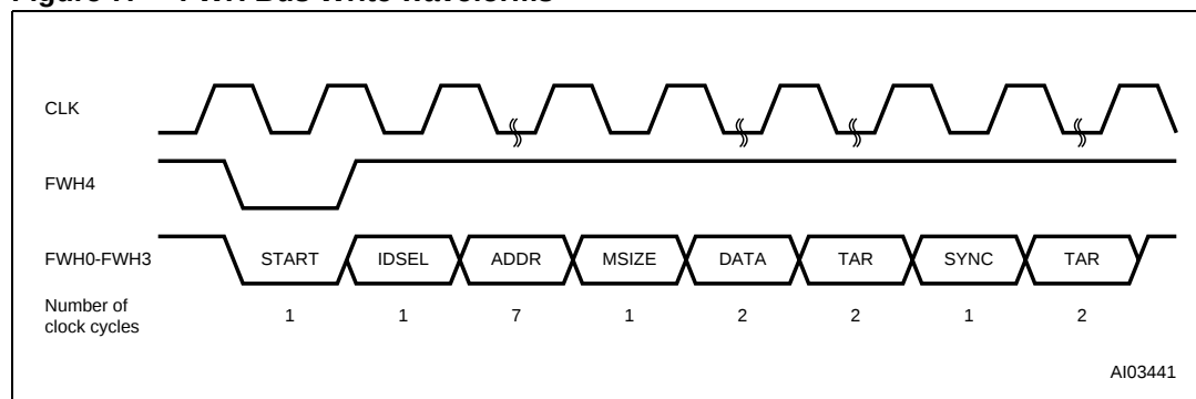
Figure 7. FWH Bus Write waveforms
