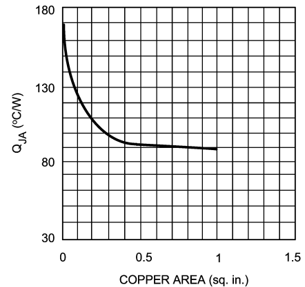
FIGURE 3. \theta_{JA} vs. Copper (1 ounce) Area for PSOP Package
