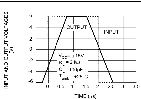
Figure 15. Voltage follower large signal pulse response
