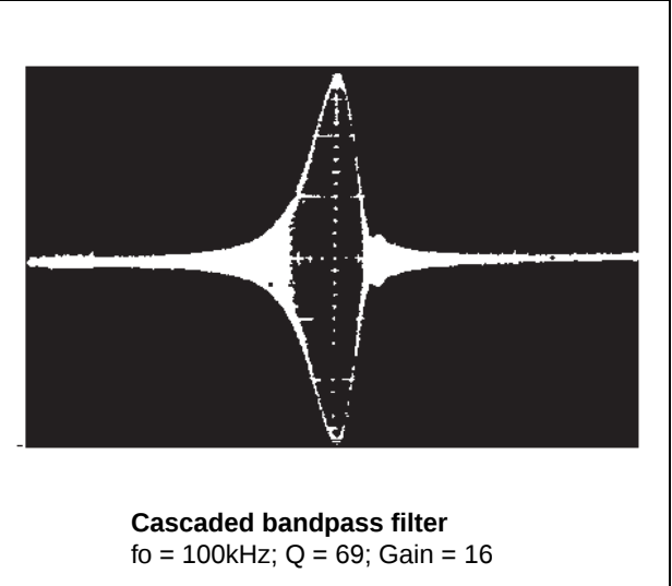
Figure 24. Output B
