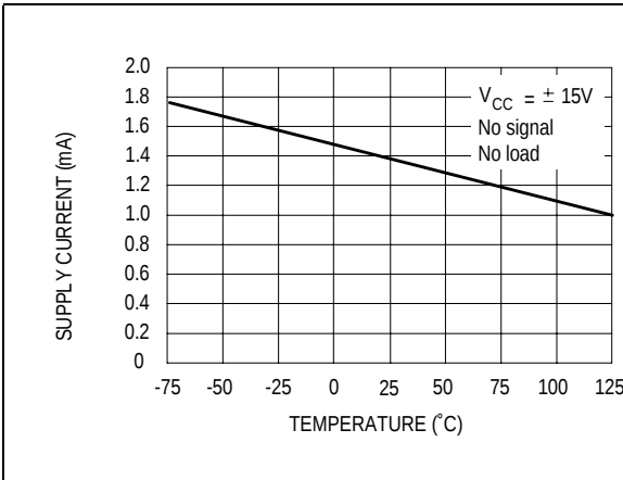
Figure 12. Supply current per amplifier versus free air temperature
