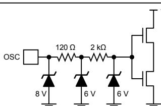
Figure 18f. OSC Input
