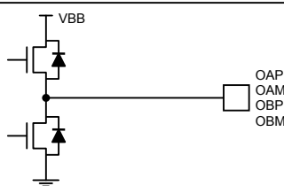
Figure 18i. Phase Outputs
