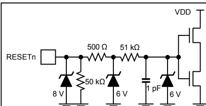
Figure 18g. RESETn Input
