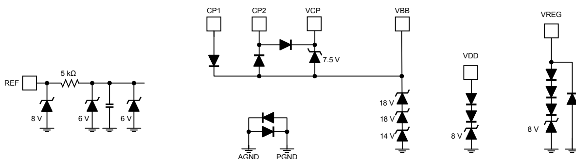
Figure 18a. Supplies and Reference
