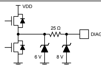
Figure 18j. DIAG Output
