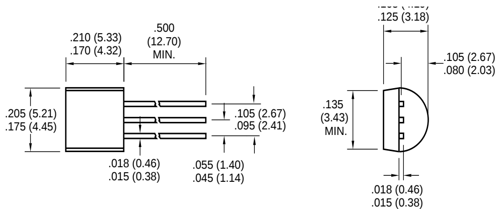
3-Pin TO-92
