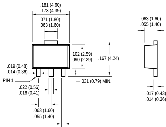
3-Pin SOT-89
