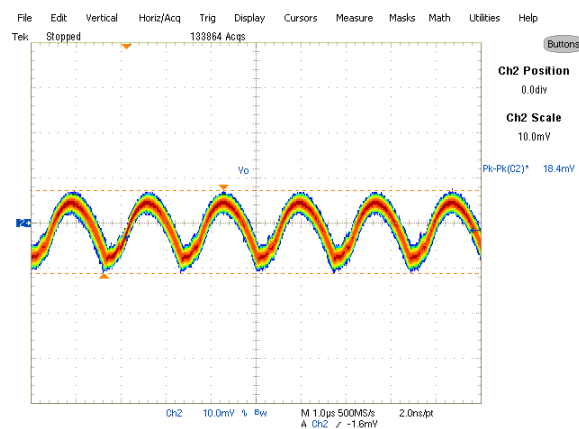
Fig. 10: Output Voltage Ripple, 8A load Ch 2 : V_{out}
