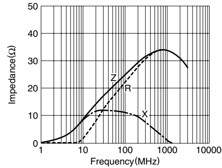
MPZ1608S121A
