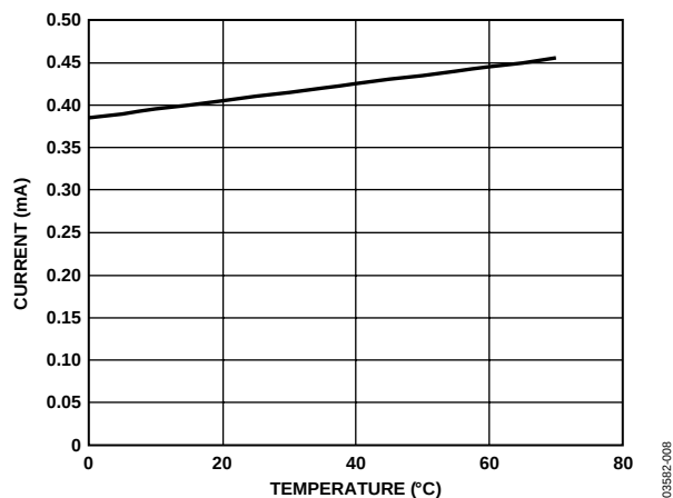
Figure 9. Typical Supply Current vs. Temperature
