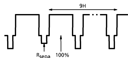
Sync. separation input
