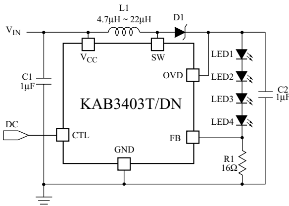
Figure6. Using a DC Signal to CTL pin.
