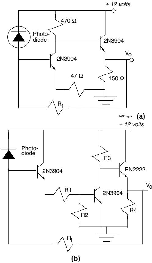
Figure 9.5 Fiber optic receivers using a discrete bipolar transistor.
