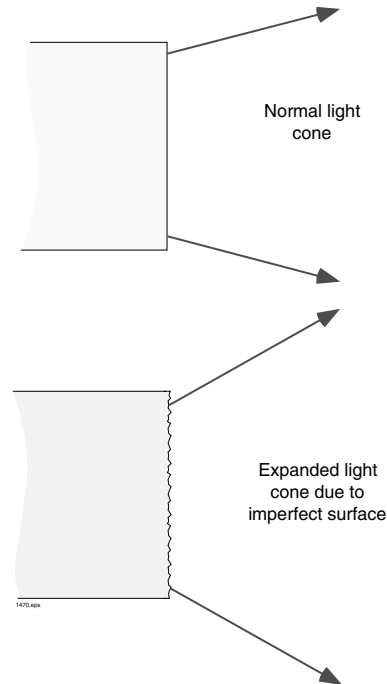
Figure 6.1 (Top) Fiber with a perfectly flat termination, arrows depicting the cone of light exiting the fiber core. (Bottom) A poor fiber polish/termination showing the resultant increased divergence of exiting light rays.
