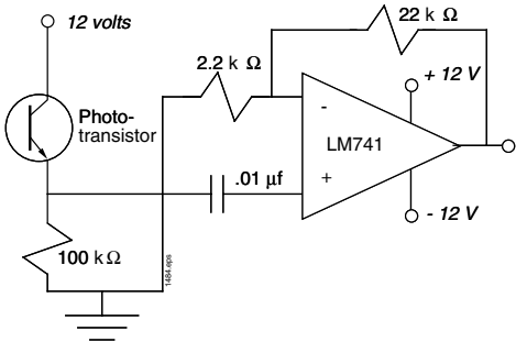
Figure 9.6 (a)Inverting phototransistor CMOS receiver; (b)non-inverting receiver with AC-coupled buffer amplifier.
