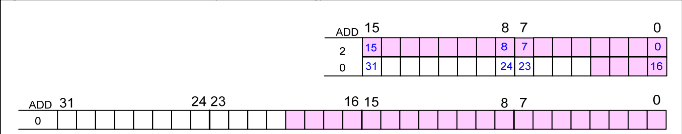
Figure 11-4. Partial Data Elements (16 to 32 bits long)
