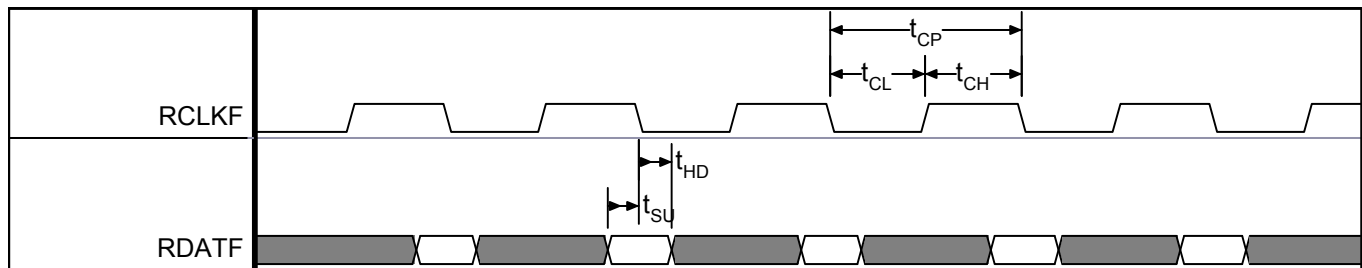
Figure 14-4. Receive Framing Timing, Line Side with LIU Not Used
