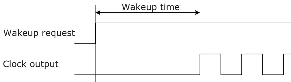
Figure 36-2. Wake-up time definition.
