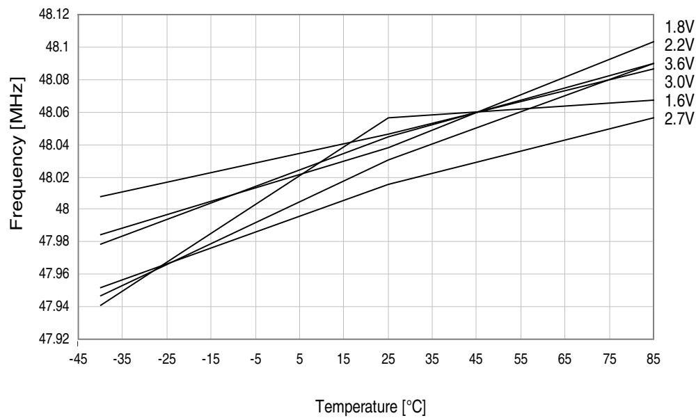
Figure 37-72. 48MHz internal oscillator frequency vs. temperature. DPLL enabled, from the 32.768kHz internal oscillator.
