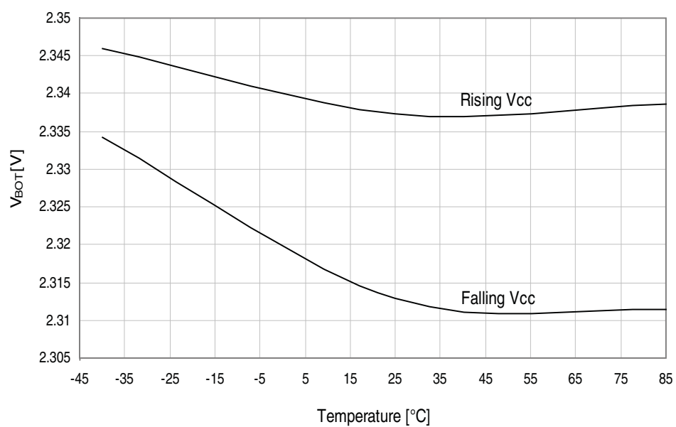
Figure 37-50. BOD thresholds vs. temperature.
