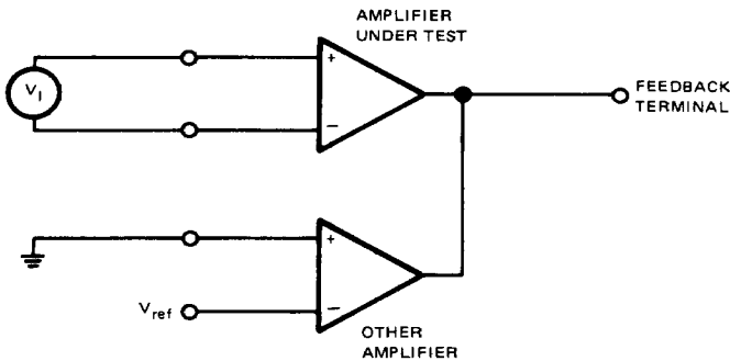
FIGURE 1 — AMPLIFIER CHARACTERISTICS
