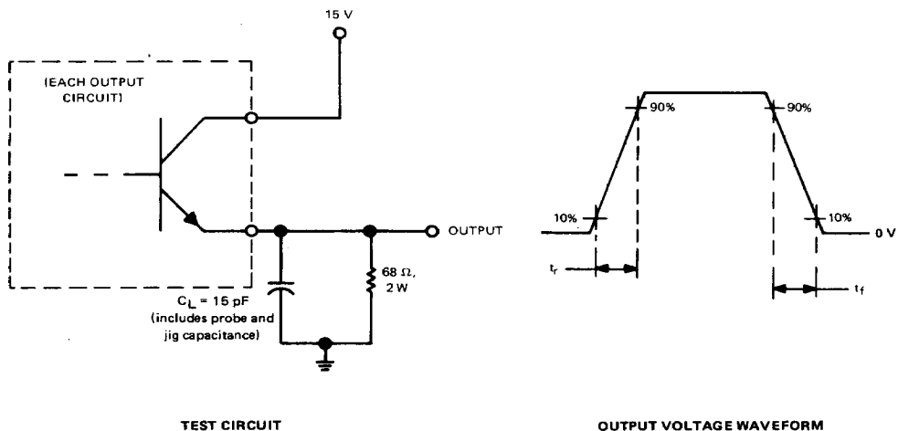
TEST CIRCUIT
