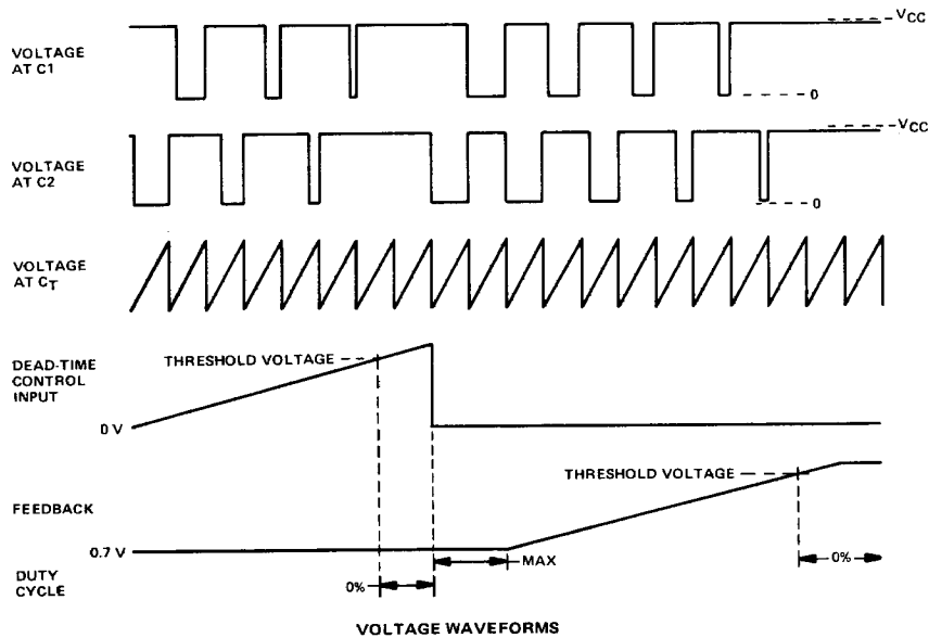
FIGURE 2—OPERATIONAL TEST CIRCUIT AND WAVEFORMS
