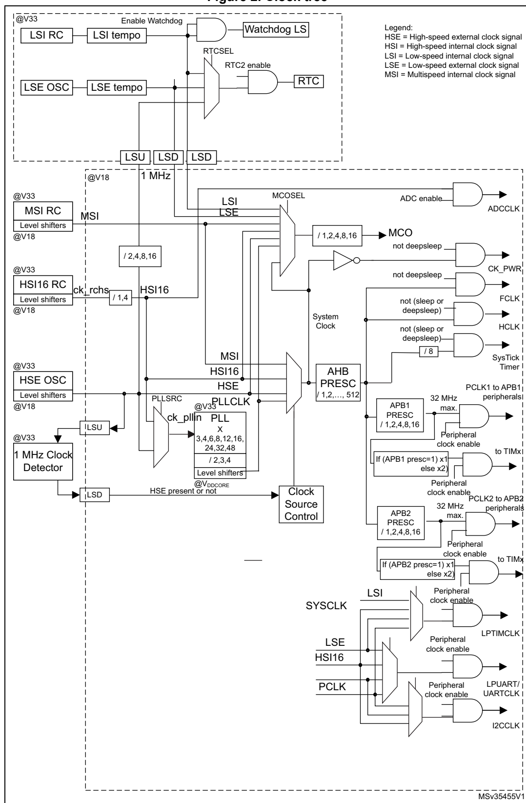
Figure 2. Clock tree
