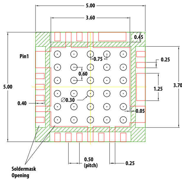
Land Pattern
