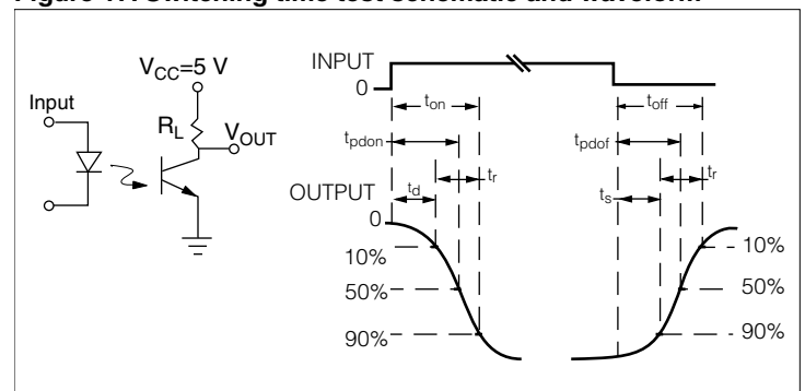
Figure 17. Switching time test schematic and waveform
