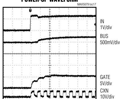
POWER-UP WAVEFORM
