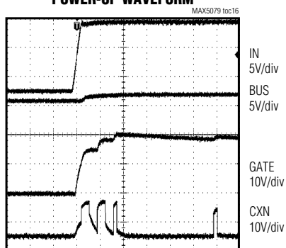
POWER-UP WAVEFORM
