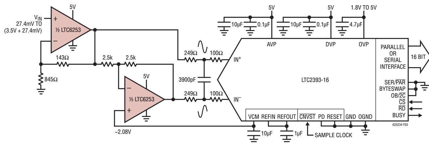
Figure 3. 5V Single Supply 16-Bit ADC Driver
