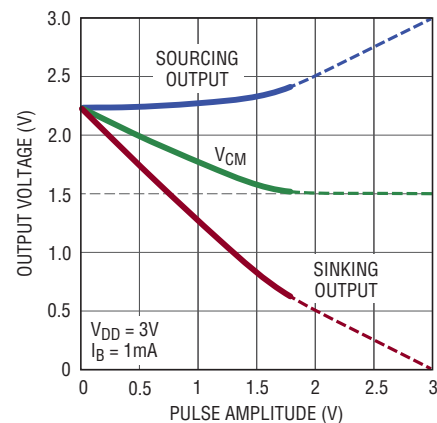
Figure 9. Output Voltages and Common Mode vs Amplitude
