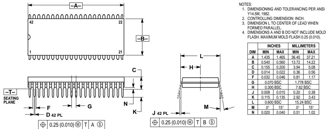
Figure 22-2. 42-Pin SDIP (Case 858)
