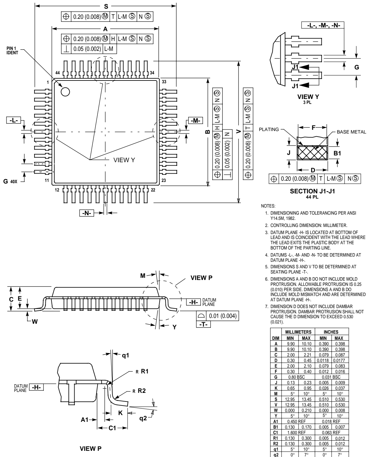
Figure 22-3. 44-Pin QFP (Case 824E)
