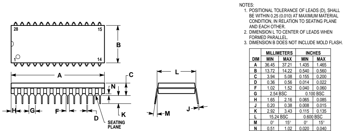
Figure 22-1. 28-Pin PDIP (Case 710)
