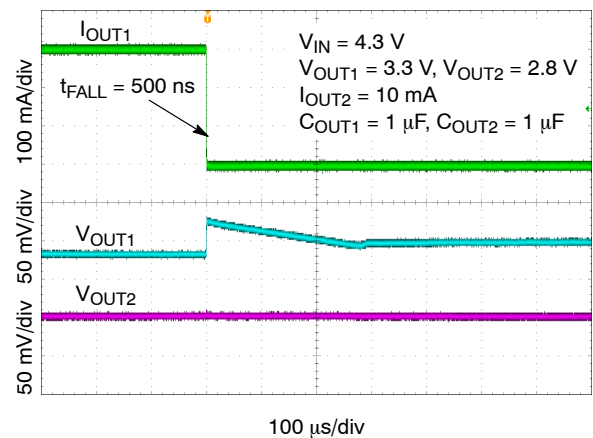
Figure 47. Load Transient Response – 3.3 V – Falling Edge, I_{OUT1} = 300 mA to 100 \mu A
