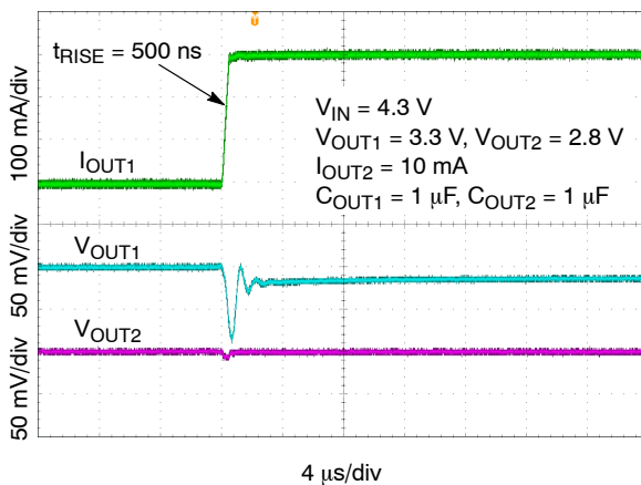
Figure 46. Load Transient Response – 3.3 V – Rising Edge, I_{OUT1} = 100 \mu A to 300 mA
