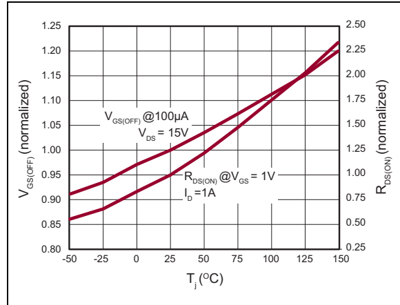
FIGURE 2-6: V_{GS(OFF)} and R_{DS(ON)} Variation with Temperature.
