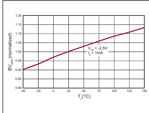
FIGURE 2-4: BV_{DSX} Variation with Temperature.
