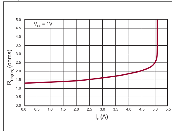
FIGURE 2-5: On-resistance vs. Drain Current.
