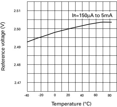
Temperature Drift
