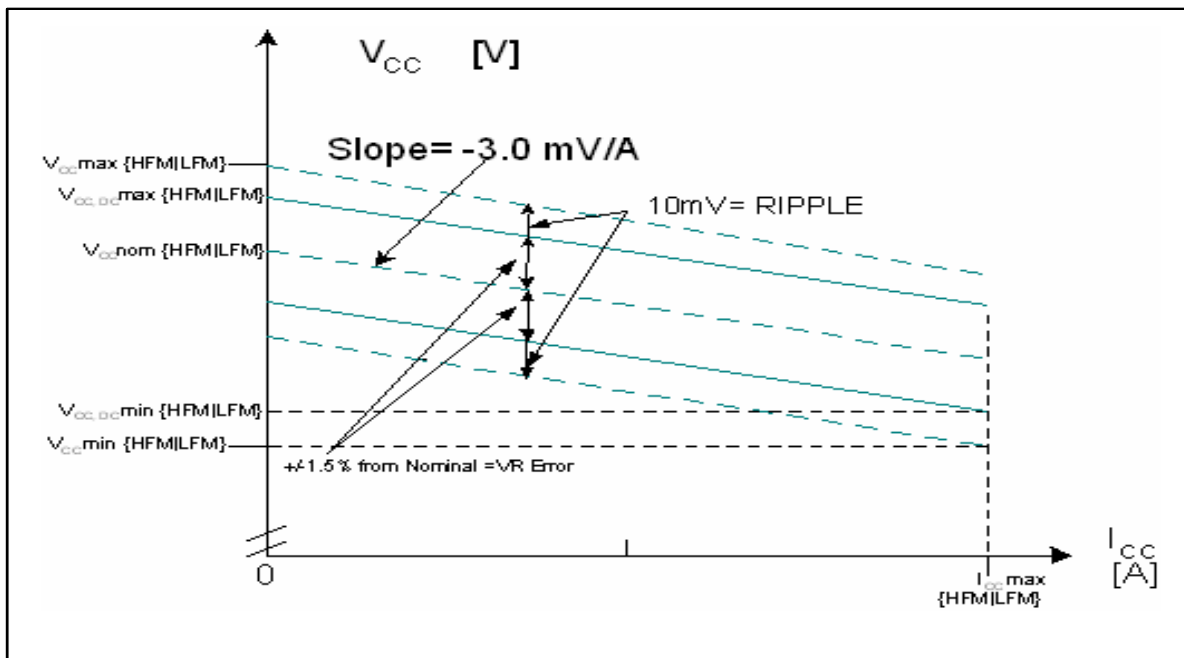
Figure 3-1. Active VCC and ICC Load Line
