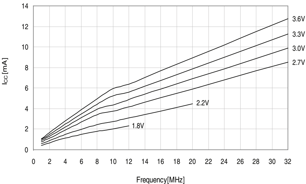
Figure 33-287. Active supply current vs. frequency. f_{SYS} = 1 - 32MHz external clock, T = 25^{\circ}C .
