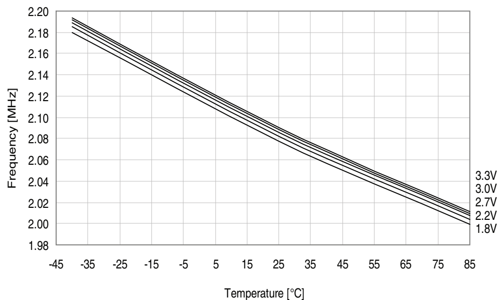
Figure 33-341. 2MHz internal oscillator frequency vs. temperature. DPLL disabled.
