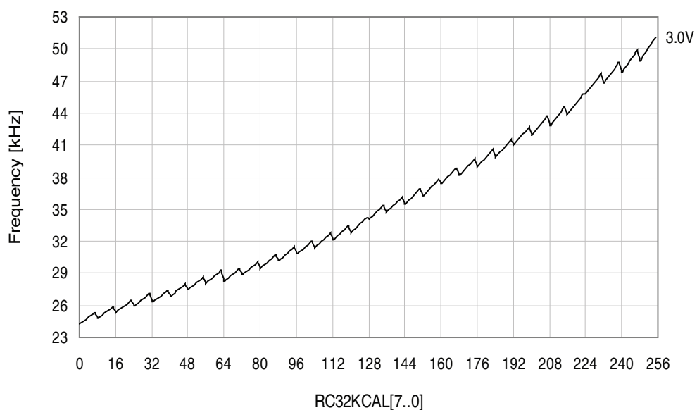
Figure 33-340. 32.768kHz internal oscillator frequency vs. calibration value. V_{CC} = 3.0V , T = 25^{\circ}C .
