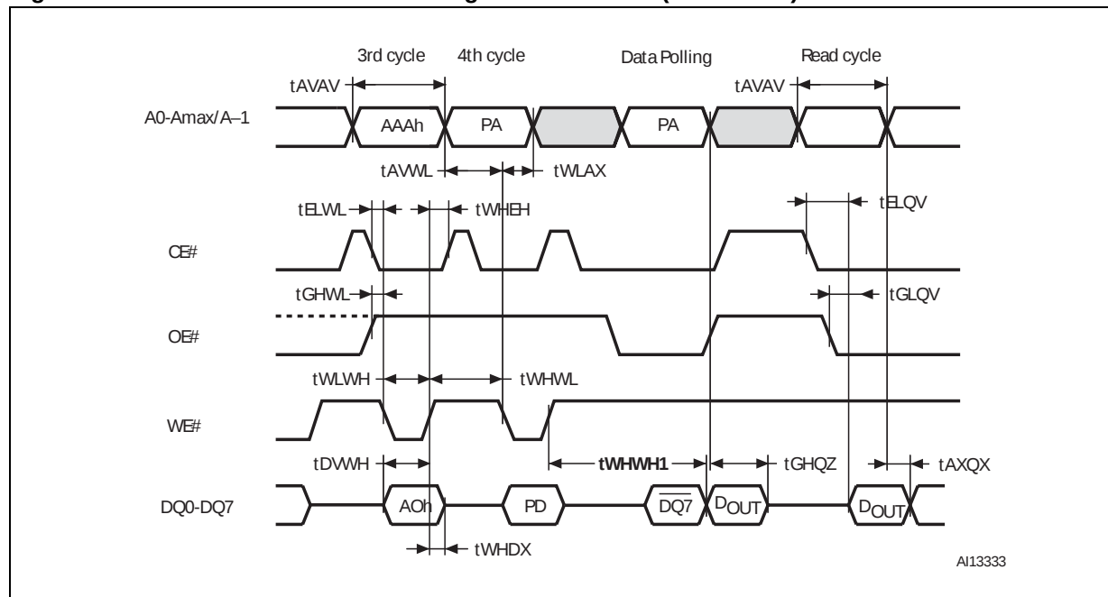
Figure 21. Write Enable Controlled Program waveforms (8-bit mode)
