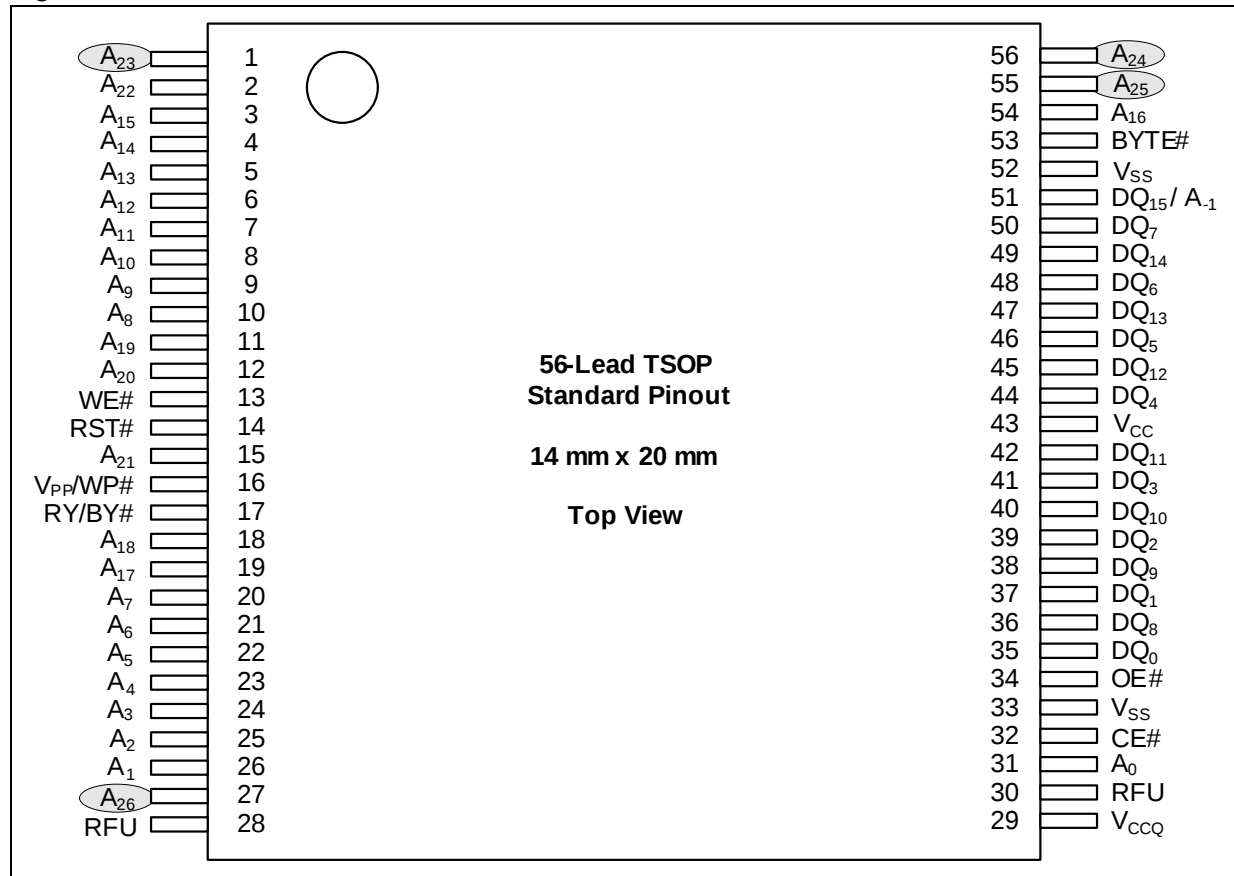
Figure 3. TSOP connections
