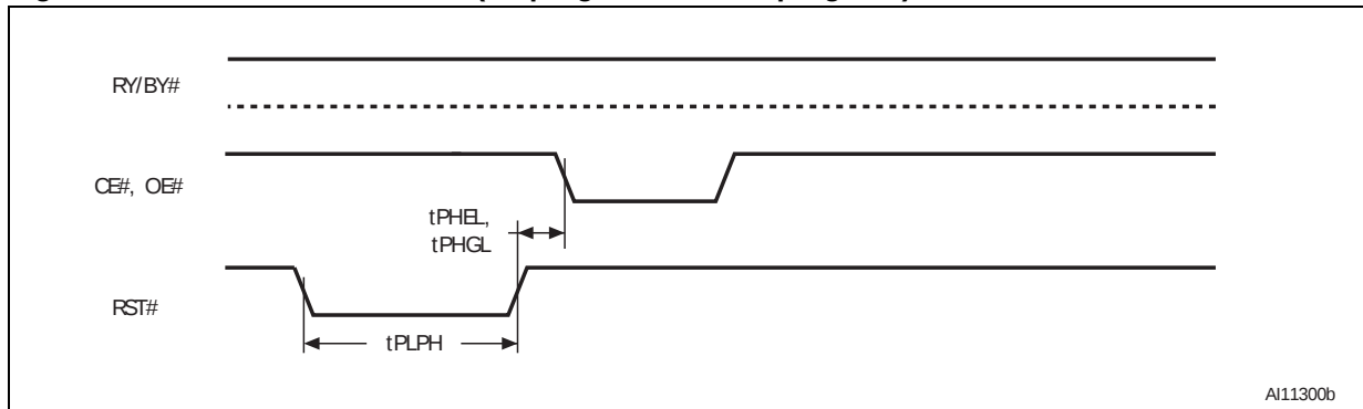
Figure 26. Reset AC waveforms (no program/erase in progress)
