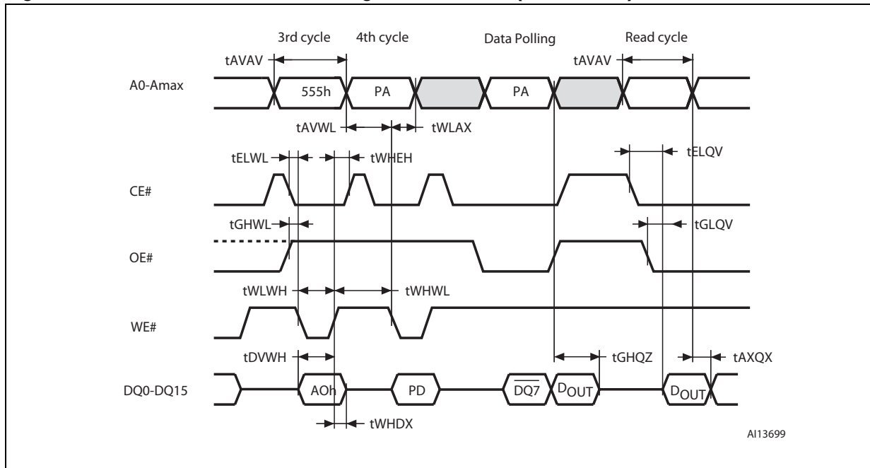
Figure 22. Write Enable Controlled Program waveforms (16-bit mode)
