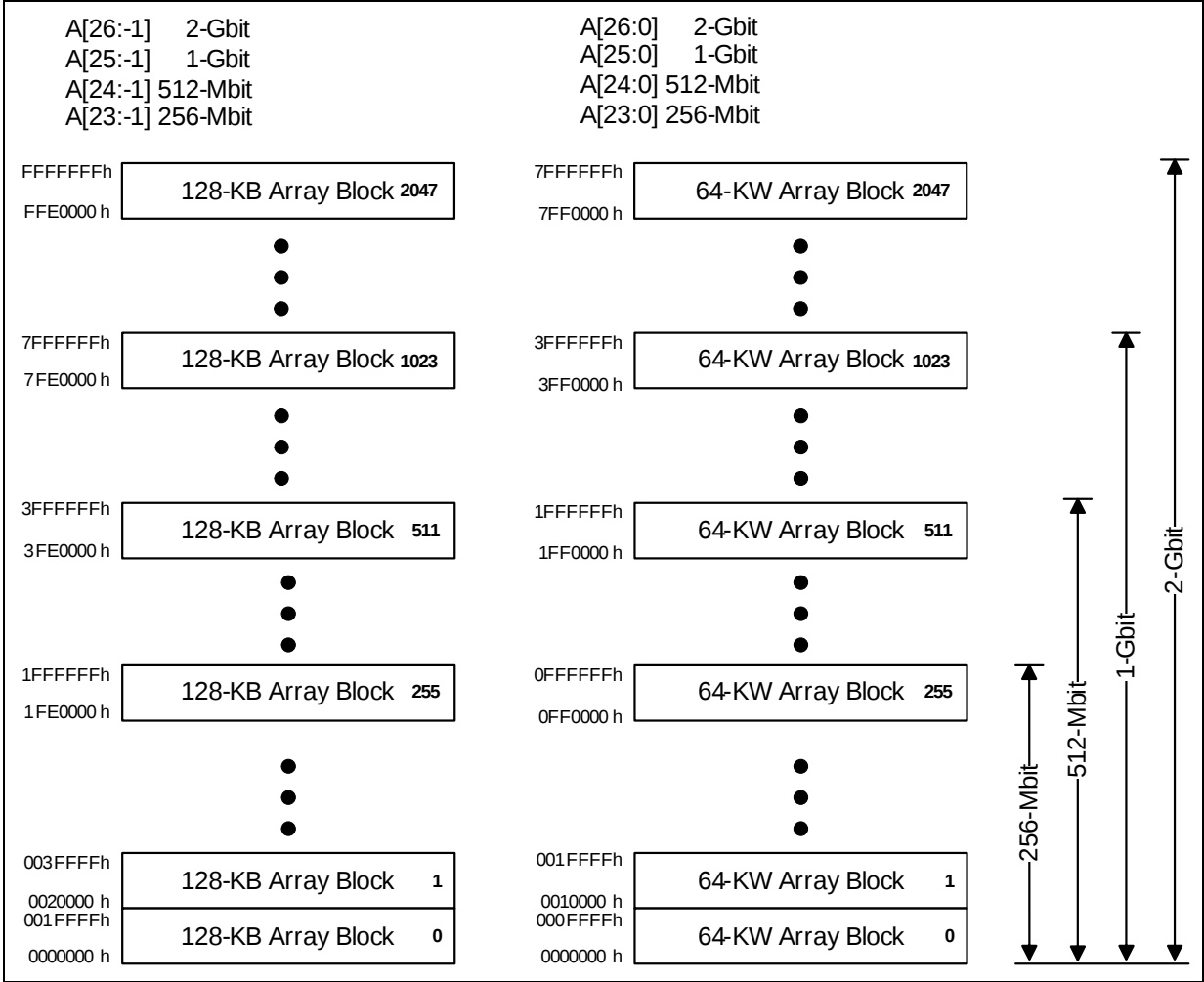
Figure 5. Block addresses
