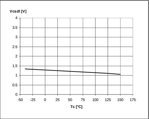
Figure 27. Low level CS_DIS voltage
