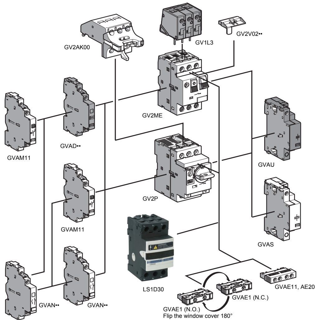
Figure 1: GV2 Accessories
