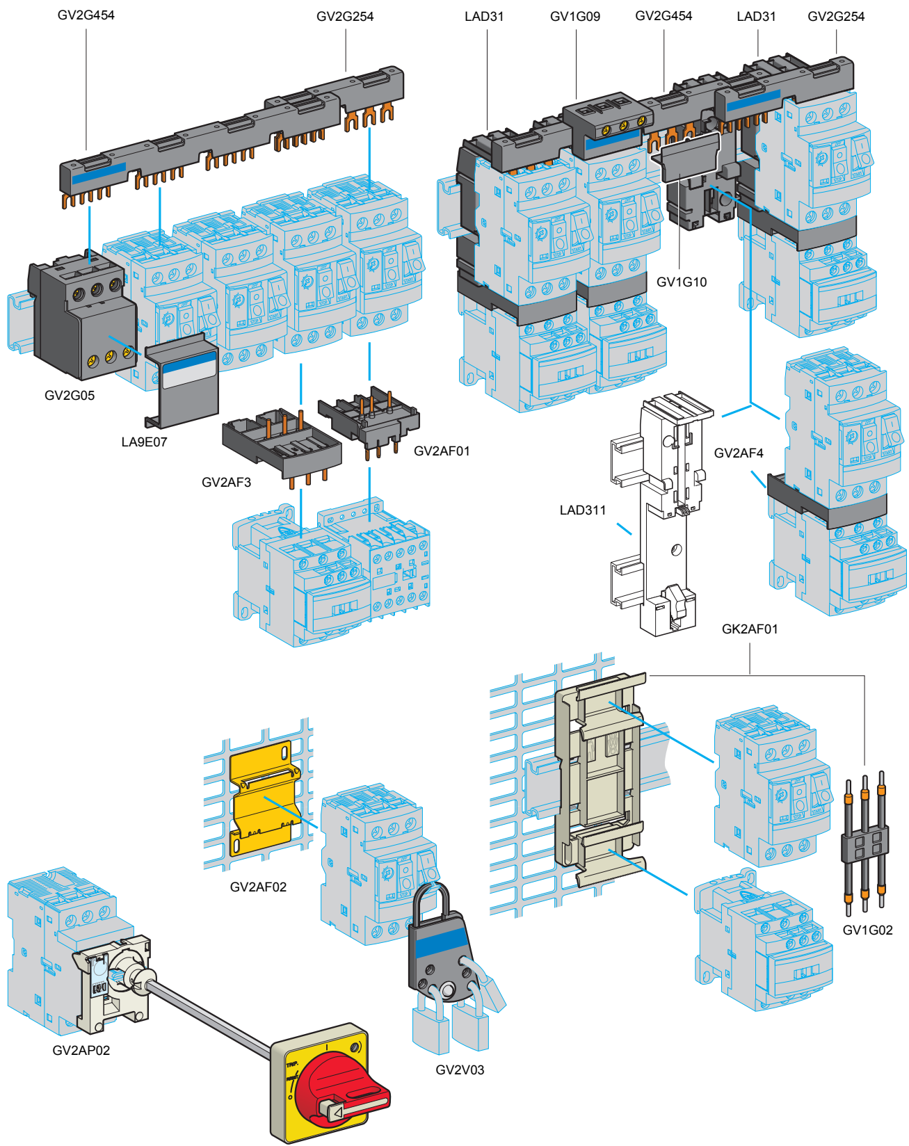
Figure 3: GV2 Accessories
