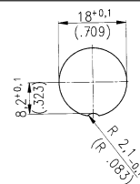
Panel Cutout
