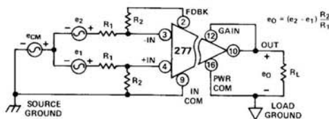
(c) Isolated Differential Configuration
