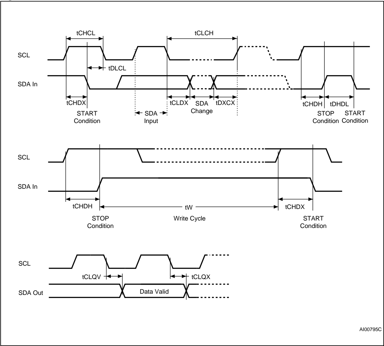
Figure 14. AC Waveforms
