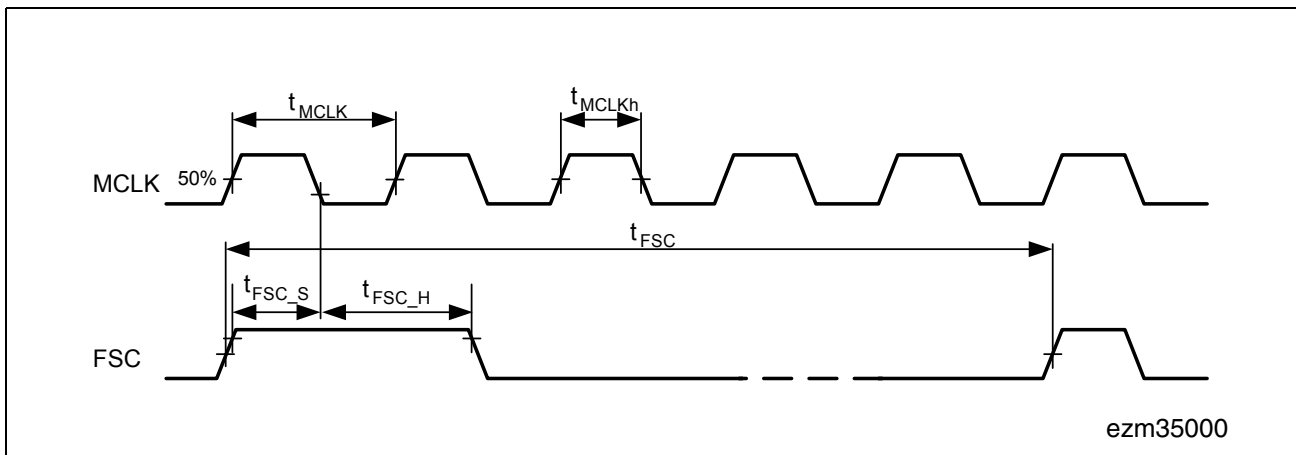
Figure 84 MCLK/FSC-Timing
