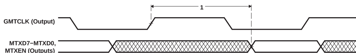
Figure 7-64. EMAC Transmit Interface Timing [GMII Operation]
