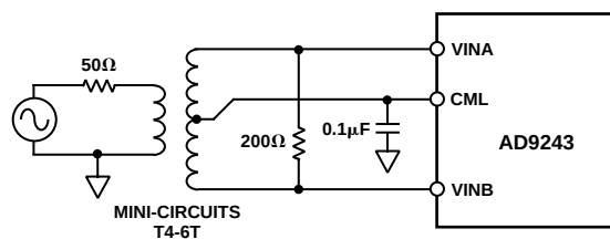
Figure 29. Transformer Coupled Input
