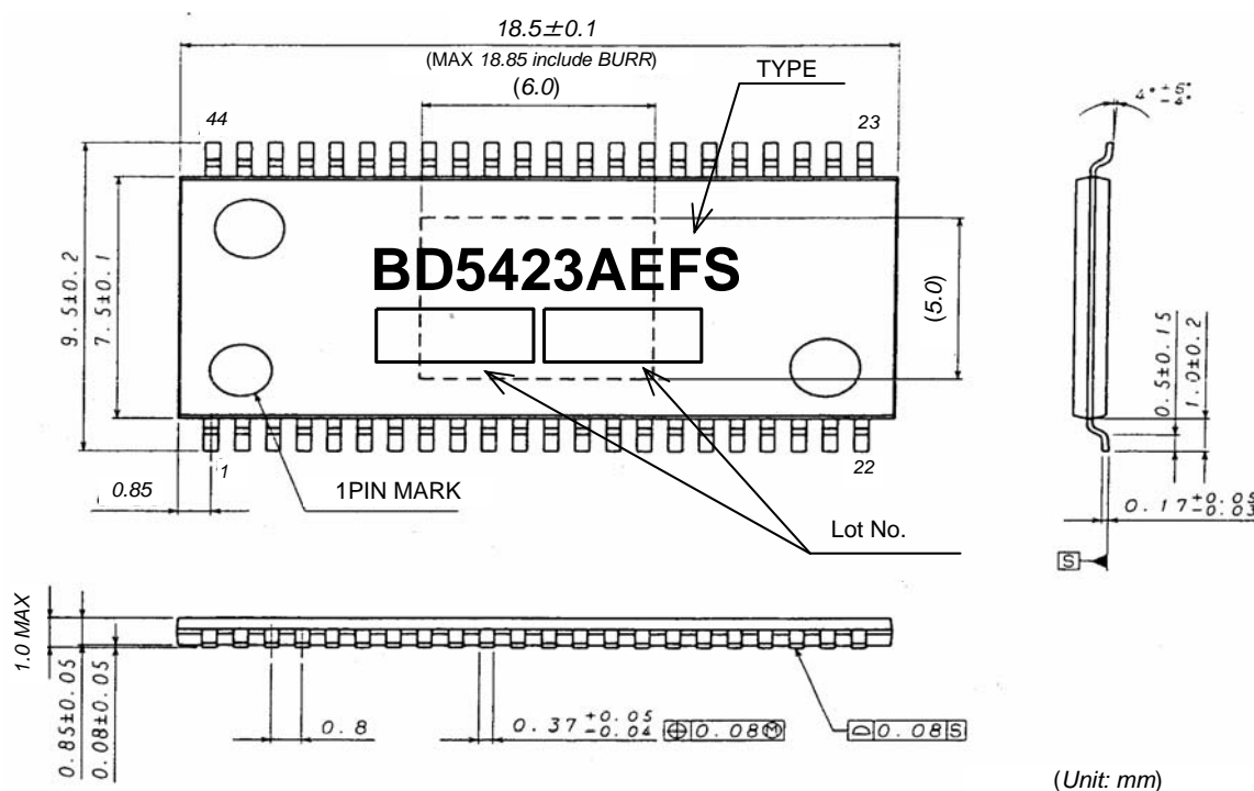
Fig. 29 Outer Dimensions and Inscriptions of HTSSOP-A44 Габариты
