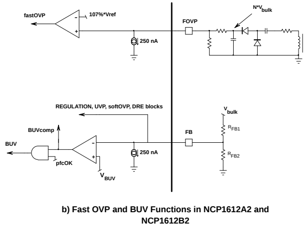
Figure 70. Bulk Under-voltage Detection
