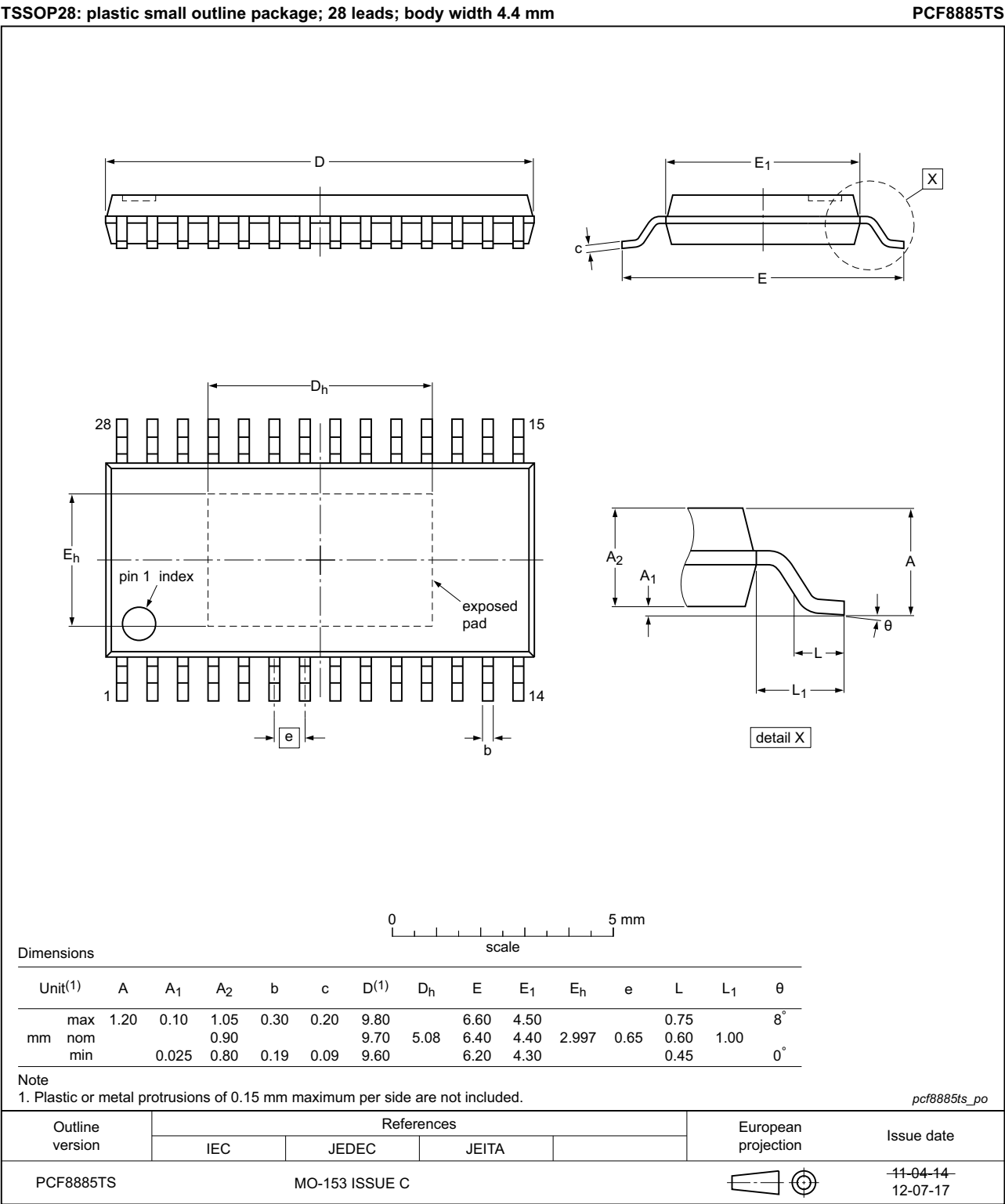
Fig 26. Package outline PCF8885TS (TSSOP28)
