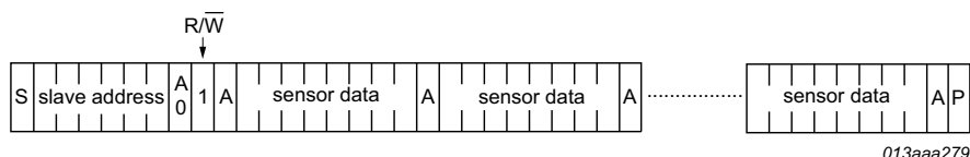
Fig 15. Continuously reading sensor data
