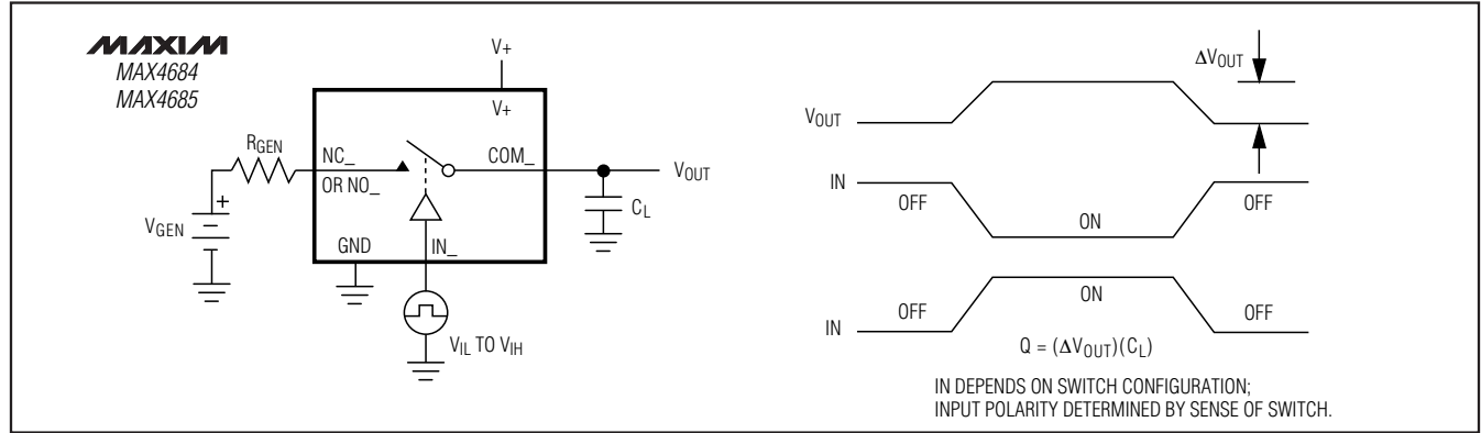
Figure 4. Charge Injection
