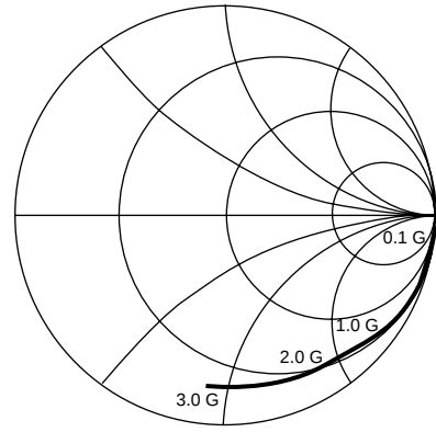
S 22 —Frequency
